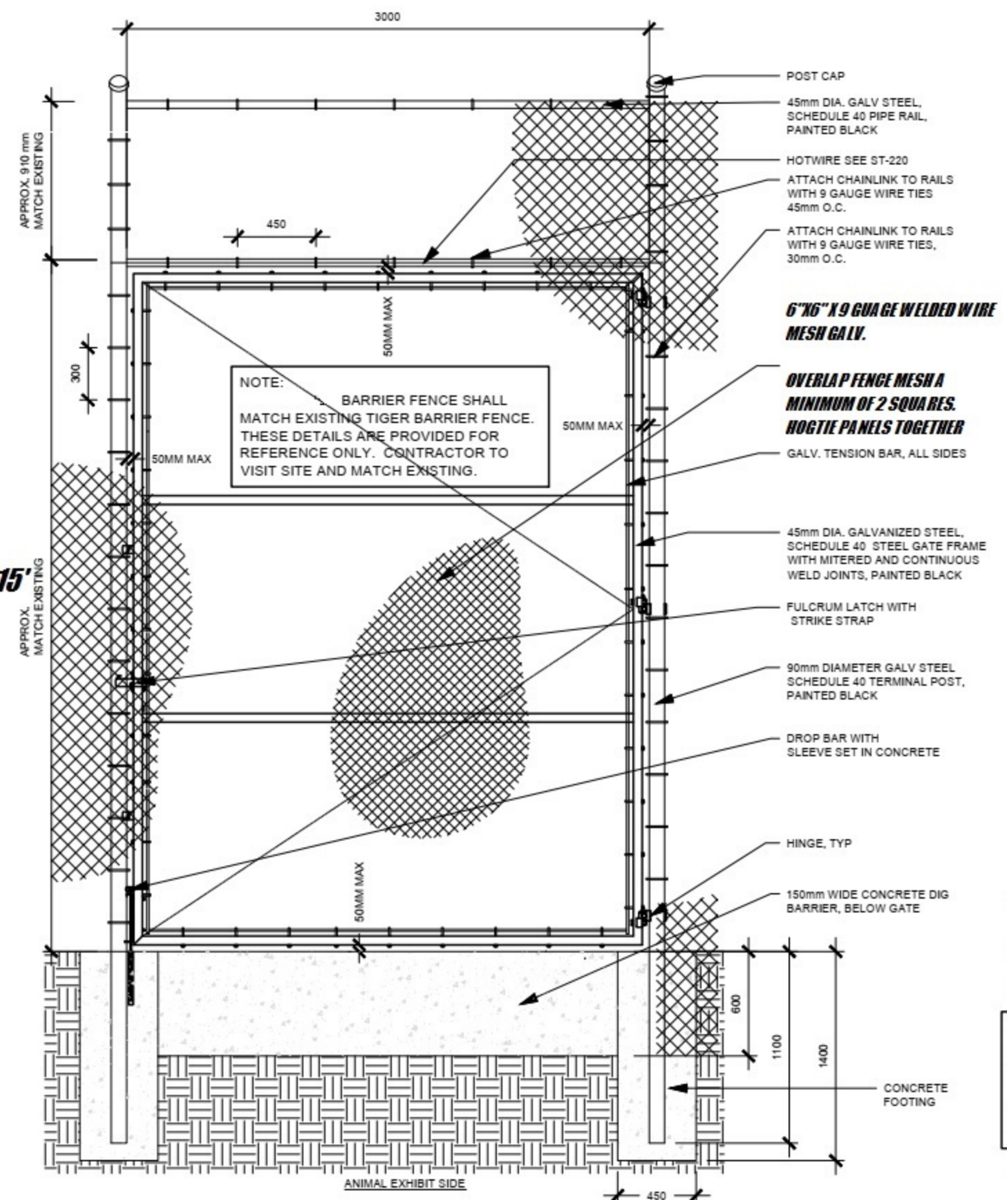
Barrier Fence Gate Elevation SCALE: 1:20
